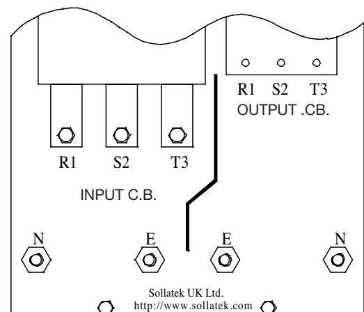
Diagram 2.6.1 Typical Terminal Arrangement
