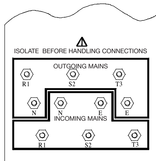
Diagram 2.6.1 Terminal Arrangement
