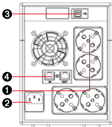
REAR PANEL 1500EU
