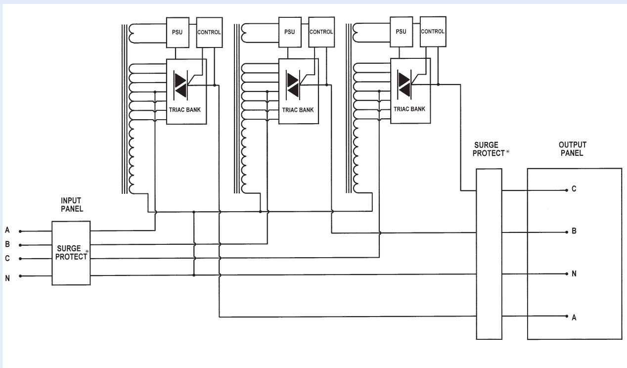
Block diagram of Sollatek Three Phase AVR
