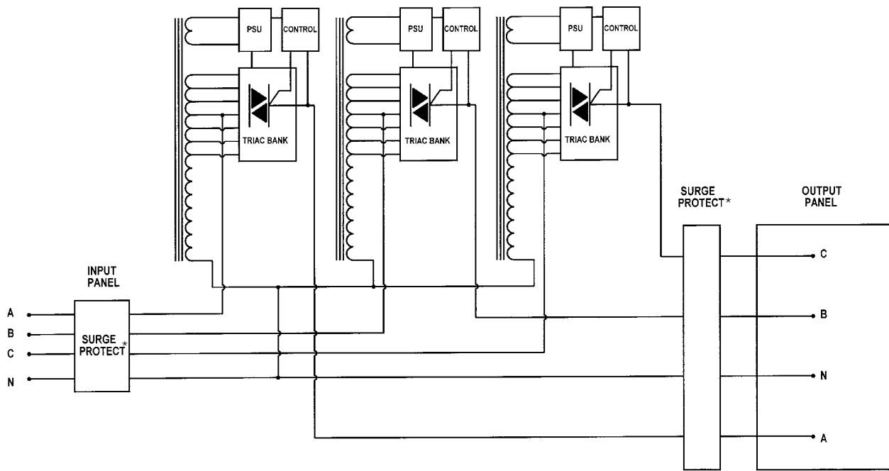
Block diagram of Sollatek 3x Series
